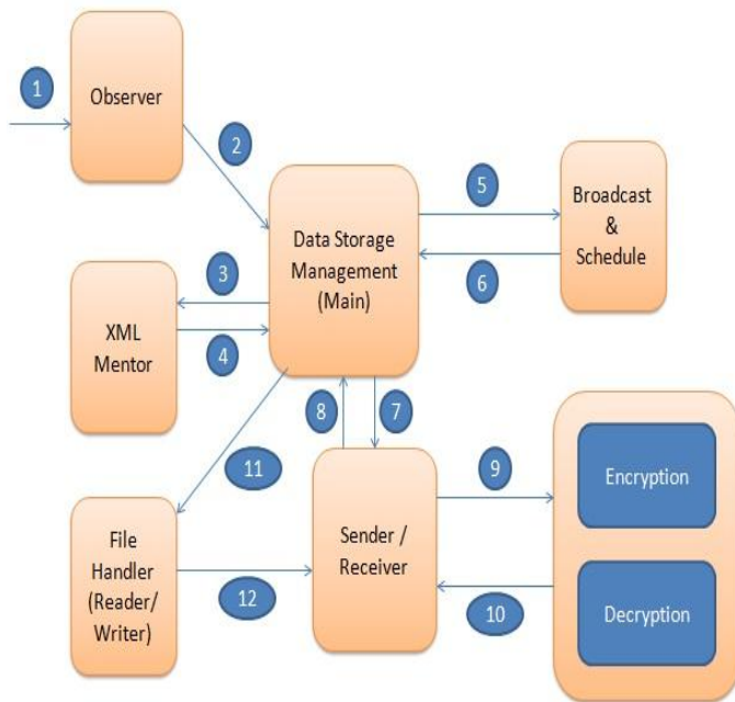
Fig -1: A secure data storage architecture system
